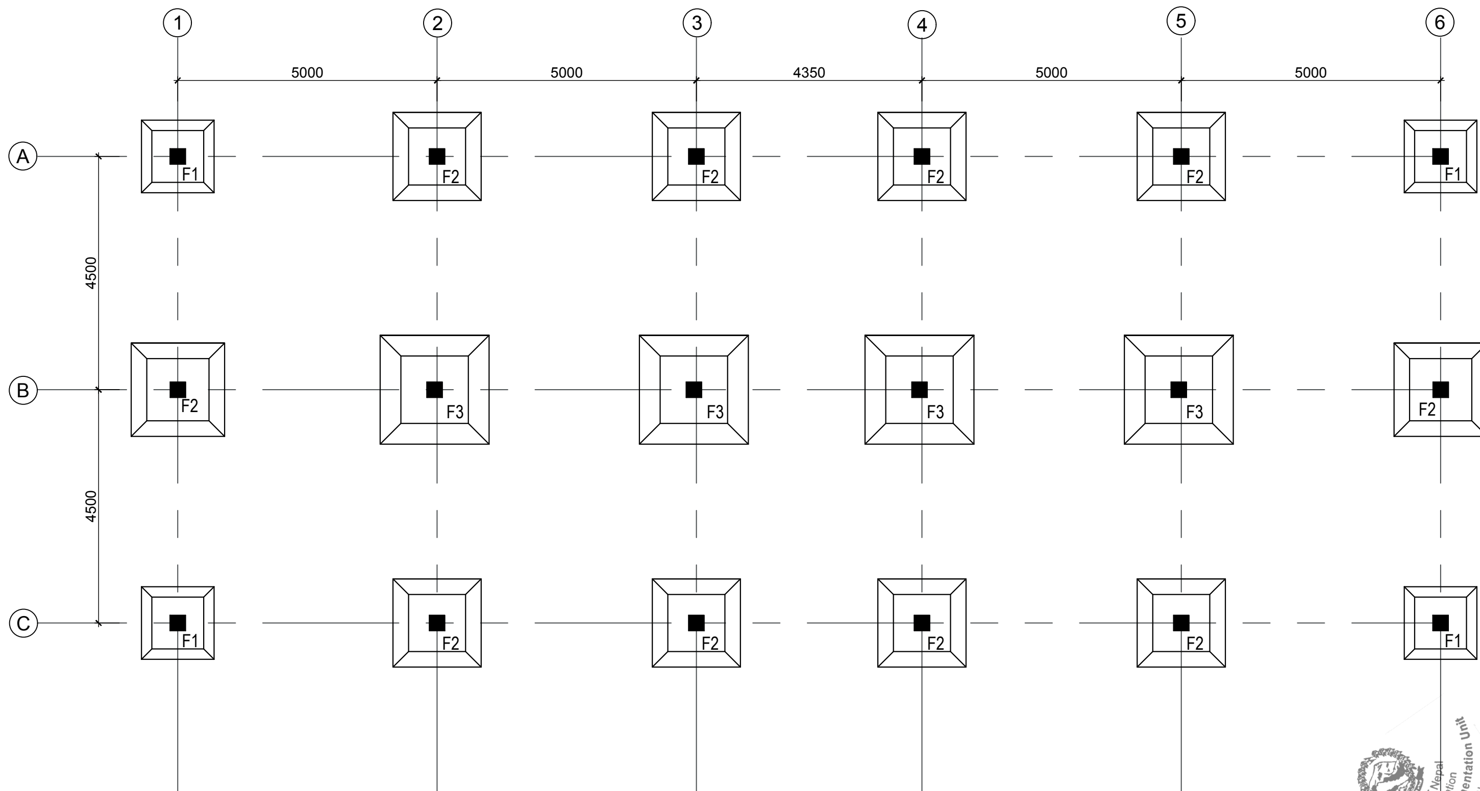
FOUNDATION PLAN
