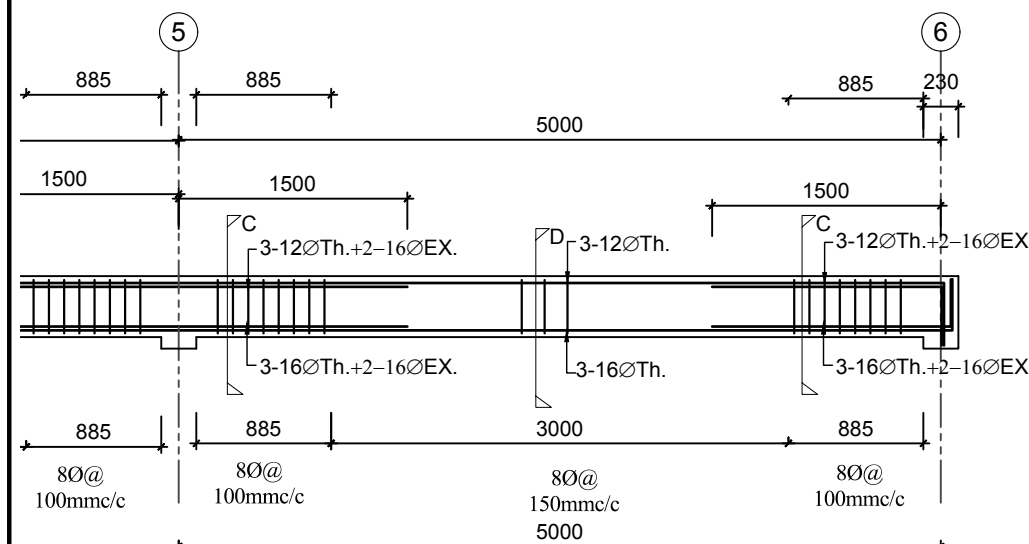
L-Section of beam along grid B' (SECONDARY BEAM)
