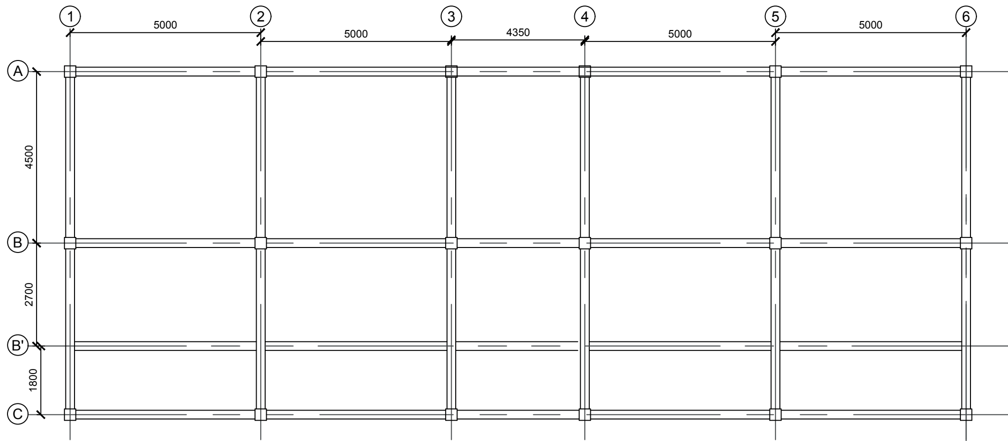
PLINTH BEAM PLAN
