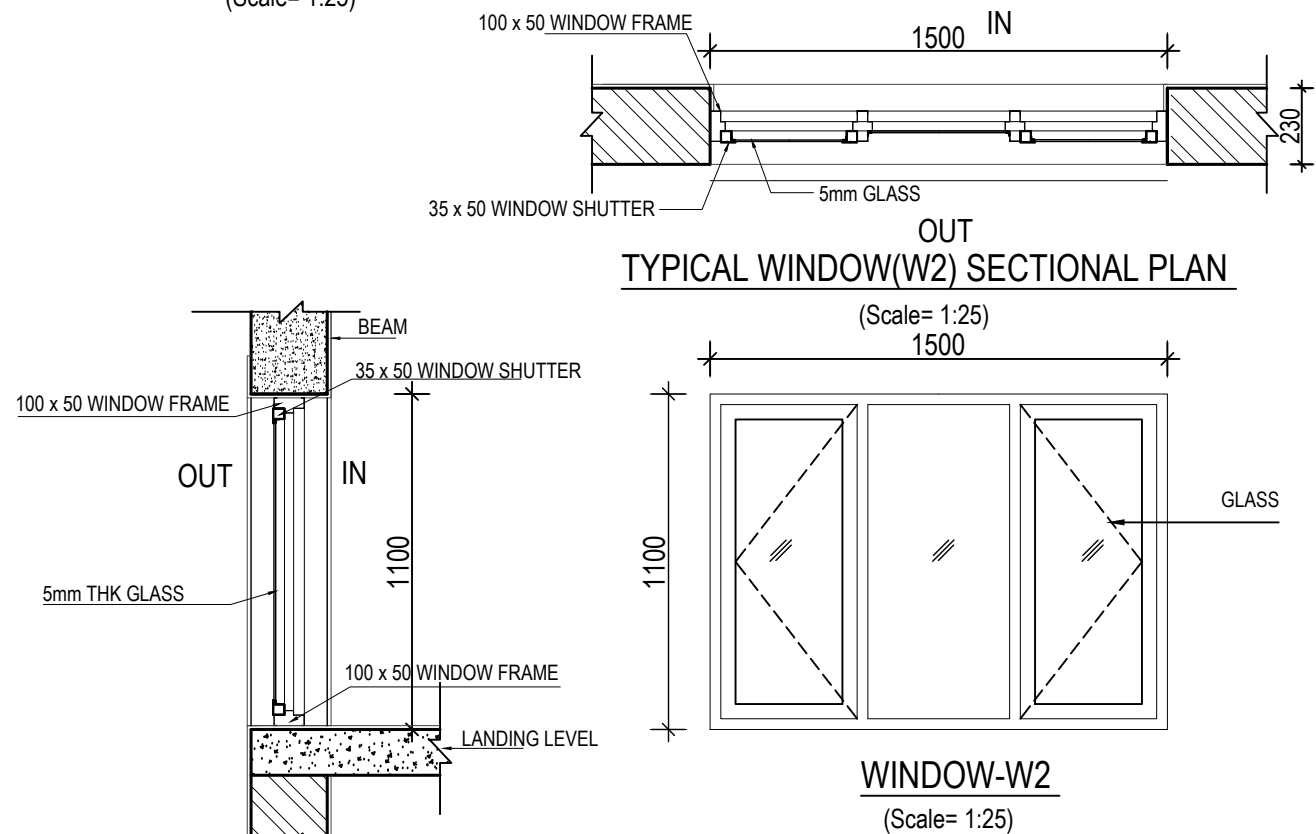
TYPICAL METAL WINDOW(W2) SECTION (Scale= 1:25)
