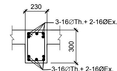
Section at D-D
