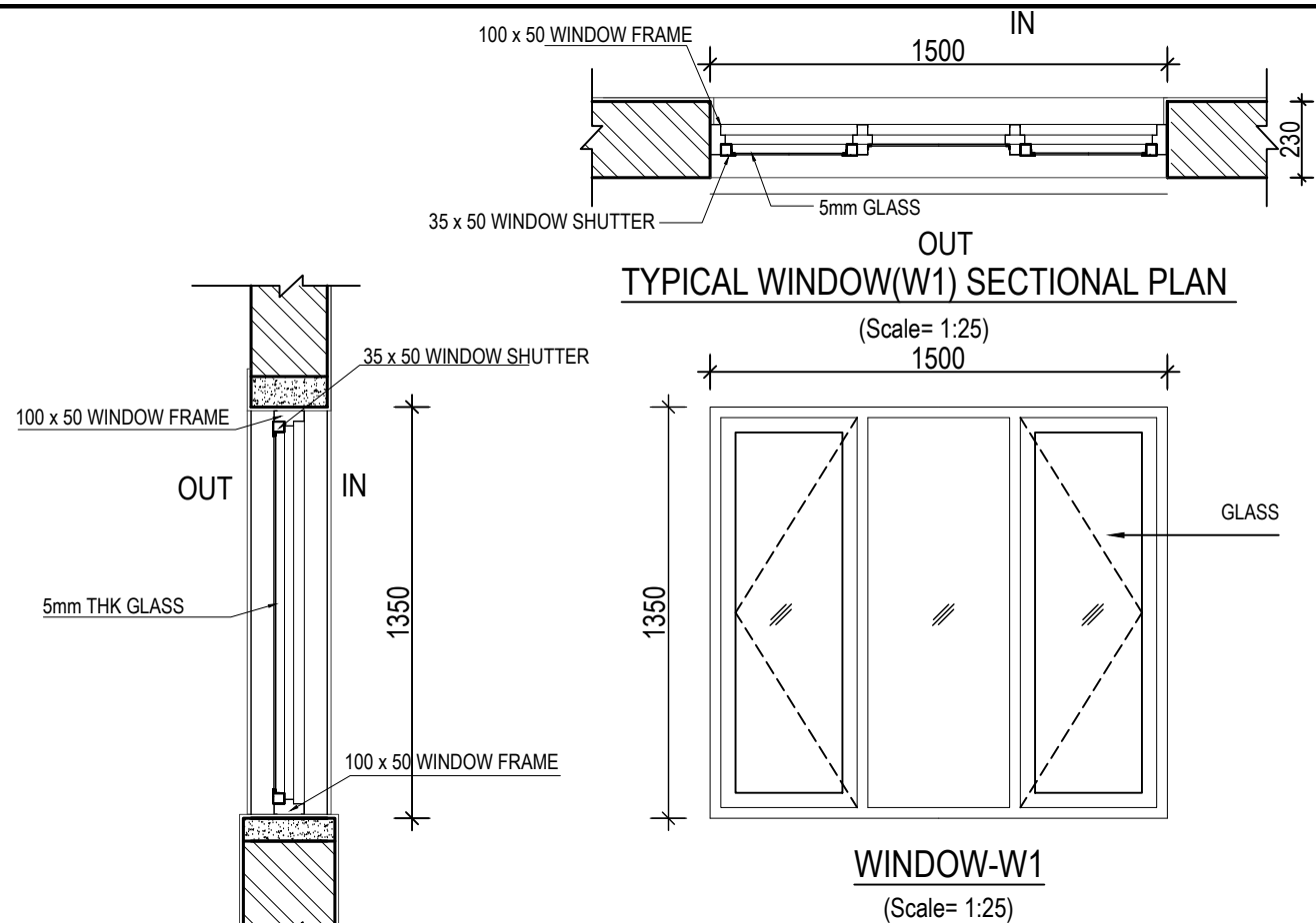
TYPICAL METAL WINDOW(W1) SECTION (Scale= 1:25)
